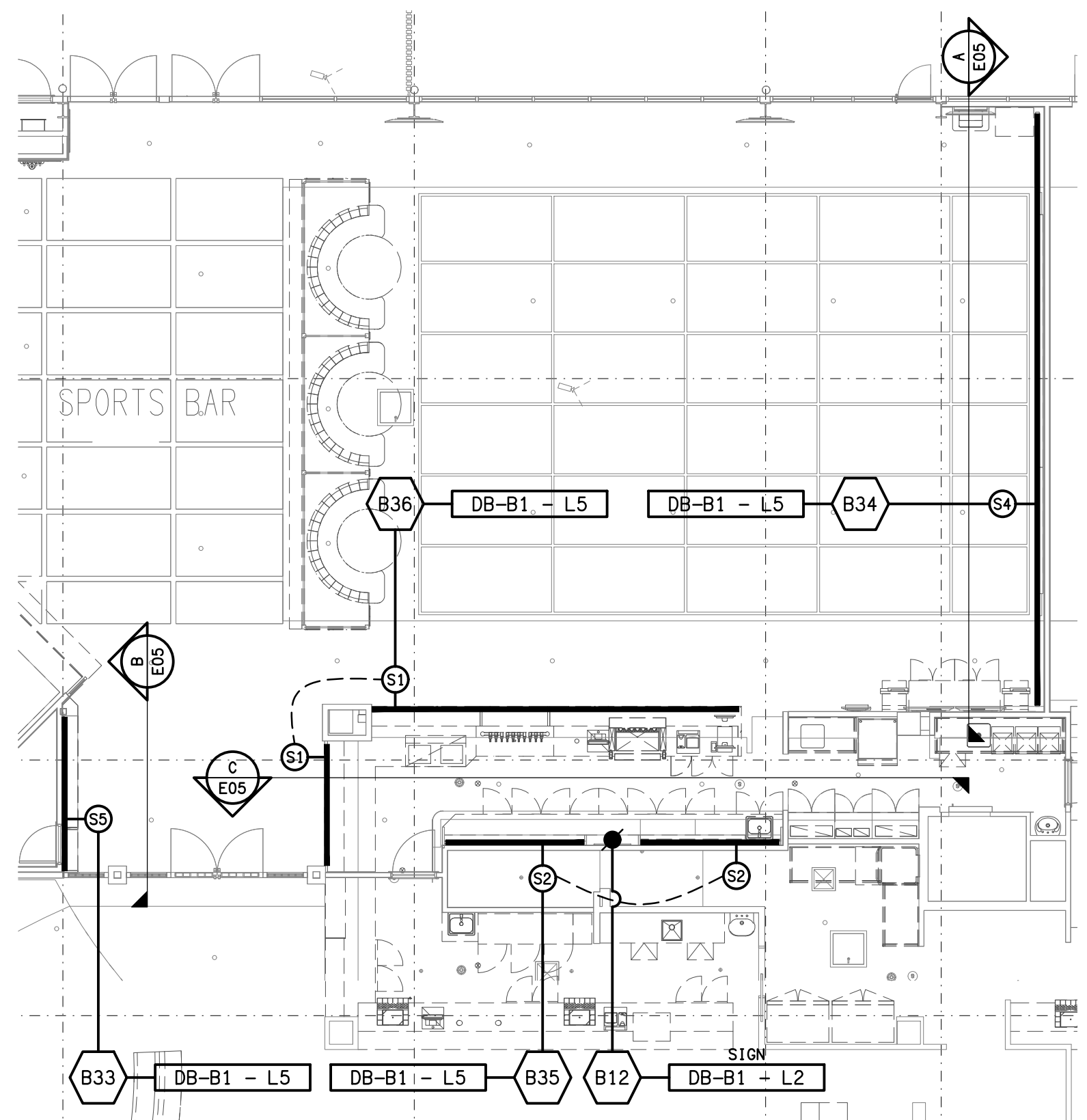
PART PLAN JOINERY LIGHTING SCALE 1:100
